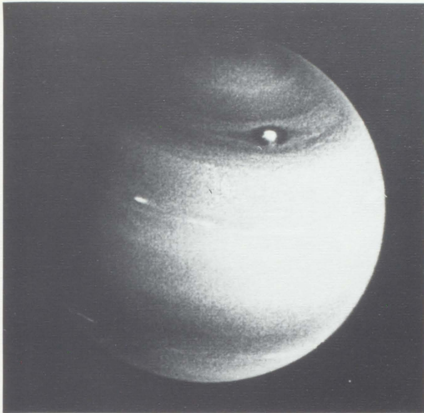
Above — The Voyager 2 capped off its 12-year tour of four planets when it skimmed 3000 miles over Neptune's north pole in August.
